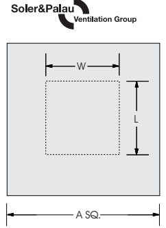
Discharge Opening
